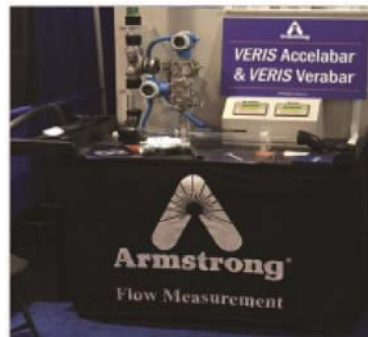
Demo- 014 VERIS Air Blower Cart Demo 2" Accelabar® and 2" Verabar® Display Dims: 58" x 26" x 60" Shipping Weight: 595lbs Shipping Dims: 66" x 35" x 75" Available for Rent
